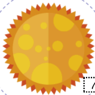
Soleil
