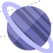
Saturne
